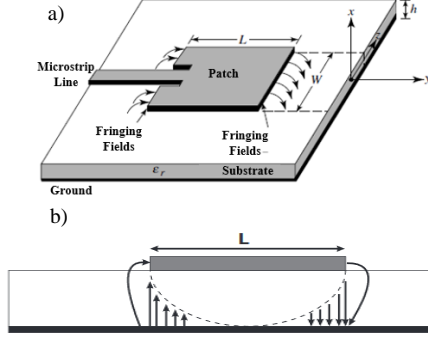
Figure 3 - a) Planar antenna with rectangular geometry representation of fringing fields excited by a microstrip line b) Side view of electromagnetic fields propagated in substrate[11]
