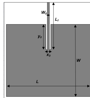
Figure 11 - Representation of antenna in CST MWS with ( W=87.4 , L=74 , W_0=2.3 , y_0=26.1 , x_0=4 , L_r=60 ) all dimensions in mm.
