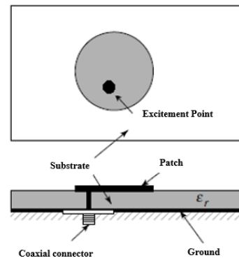
Figure 7 - Planar antenna fed by probe
