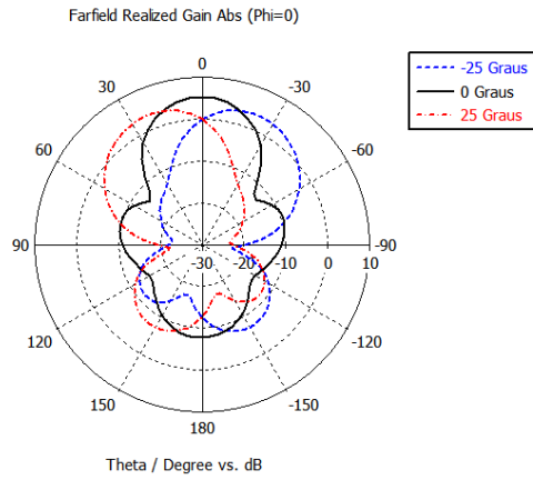
Figure 18 - Graphical representation radiation pattern in the plane and to -25^\circ , 0 and 25^\circ
