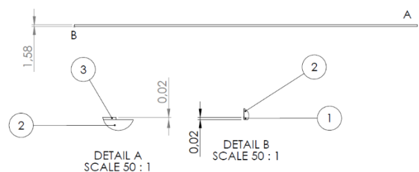
Figure 15 - Representation of the side configuration of P-ESPAR antenna with its details A and B
