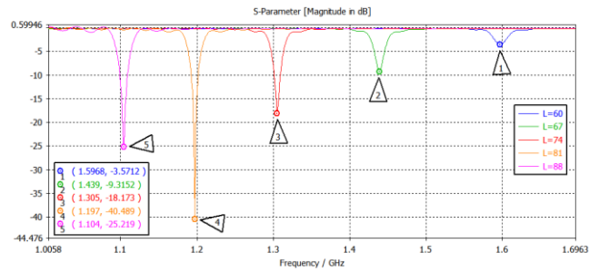
Figure 10 - Graph of change of |S_{11}|_{dB} a function of frequency for different values of L versus frequency
