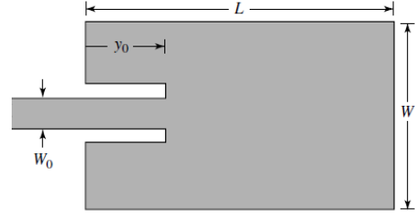
Figure 6 -Planar antenna rectangular geometry adapted to the inset feed technique[11]
