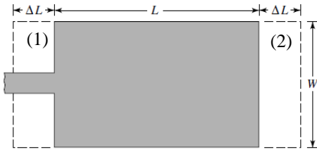
Figure 4 - Physical and effective length of the rectangular patch planar antenna[11]
