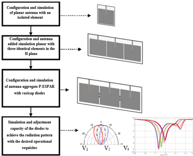
Figure 15 – a) Process study and development of P-ESPAR antenna
