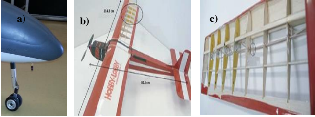
Figure 1 - Monopole \frac{1}{4} \lambda implemented in UAV; b) UAV model using a linear array of antennas embedded in the wing structure [8] c) Overview of the antenna embedded in the wing UAV [8]
