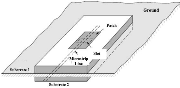
Figure 8 - Planar antenna fed by Aperture-coupled
