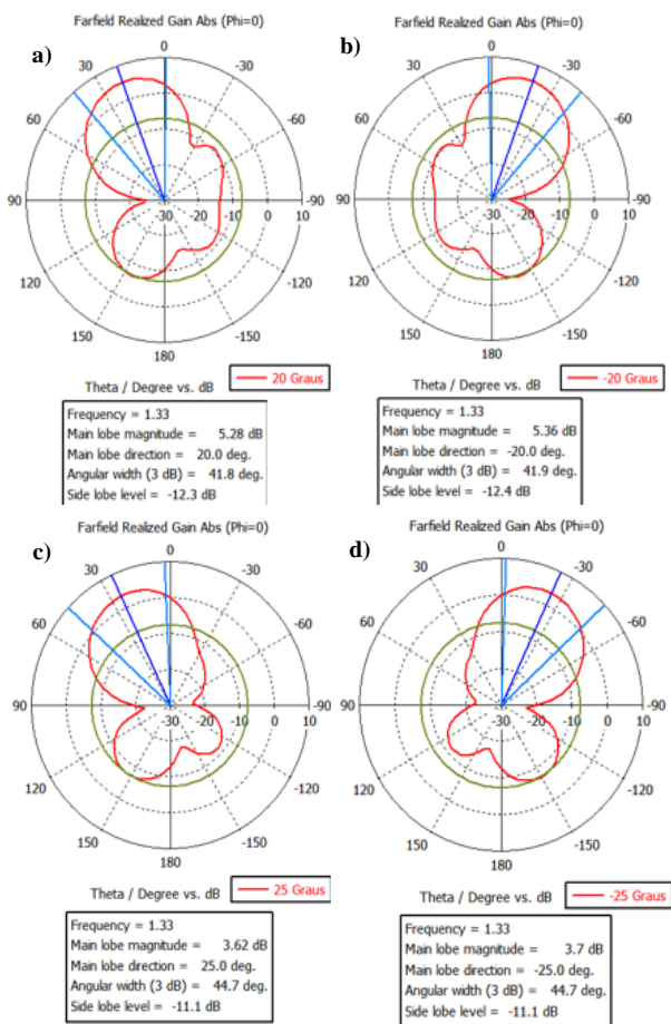
Figure 21 - Graphical representation radiation pattern in the plane E to a) 20° b) -20° c) 25° d) -25°
