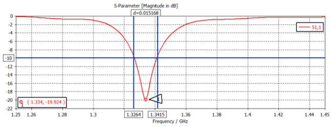
Figure 9 - Graphical representation of |S_{11}|_{dB} a function of frequency for dimensions of the planar antenna single-patch optimized
