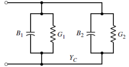
Figure 5 - Equivalent circuit of transmission line[11]
