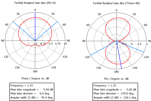
Figure 10 - Polar representation of the radiation pattern of the antenna single-patch optimized in the plane E and H
