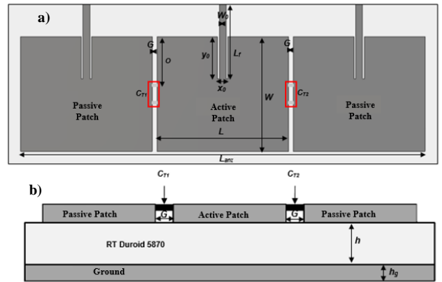
Figure 13 - a)Structure and dimensions of P-ESPAR antenna in perspective view from above b) P-ESPAR antenna on the side perspective
