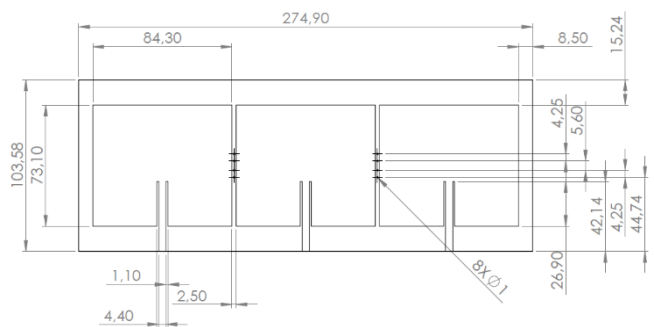
Figure 22 - Representation of the front configuration of P-ESPAR antenna
