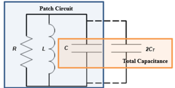
Figure 11 - Equivalent circuit of planar antenna with varicap diodes
