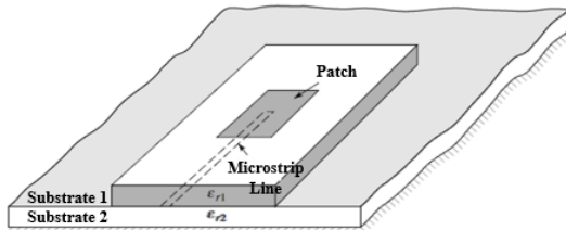
Figure 9 - Planar antenna fed by Aperture-coupled
