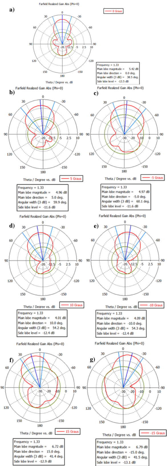
Figure 14 - Graphical representation radiation pattern in the plane E to a) 0^\circ b) 5^\circ and c) -5^\circ d) 10^\circ e) -10^\circ f) 15^\circ g) -15^\circ
