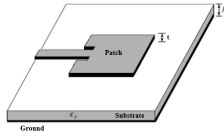
Figure 2 - Rectangular patch antenna geometry
