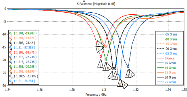
Figure 19 - Graphical representation of |S_{11}|_{dB} a function of frequency for various configurations radiation
